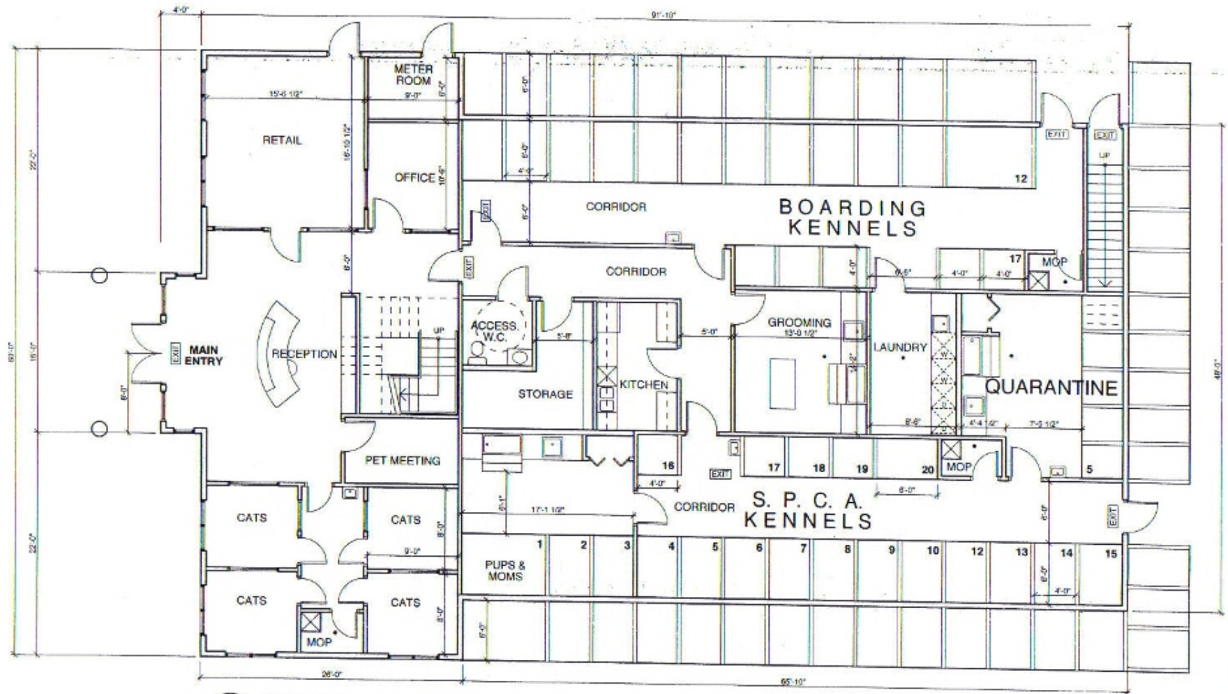
1 GROUND FLOOR (4784 sq. ft.) A2-01 SCALE: 1/8" = 1'-0"
